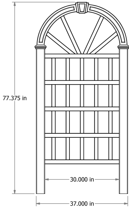
Front View SCALE 1 / 20
